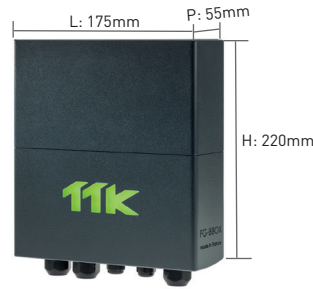
FG-BBOX-LL
