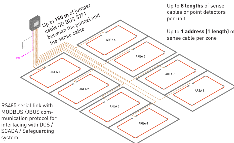
Figure 1.2.5 : Layout of FG-ALS8-OD with 8 zones
